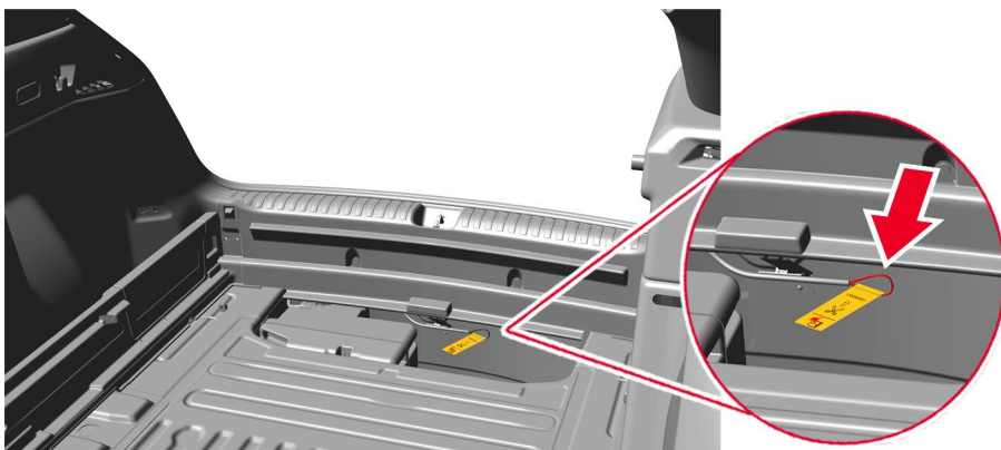
Cut-out connection in the Q4 e-tron luggage compartment under the luggage compartment floor at the rear cross panel. The yellow tag indicates the cut-out connection.
