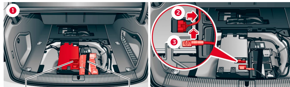
48-volt battery
