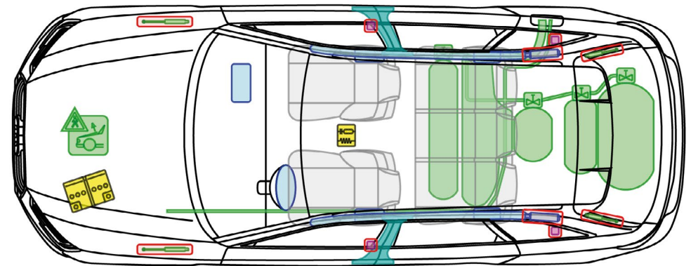
Rescue card for Audi A4 g-tron (does not comply with the current version of ISO 17840)
