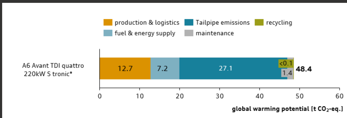
Figure 2: Global warming potential of the Audi A6 Avant TDI quattro 220kW S tronic* over the entire life cycle
